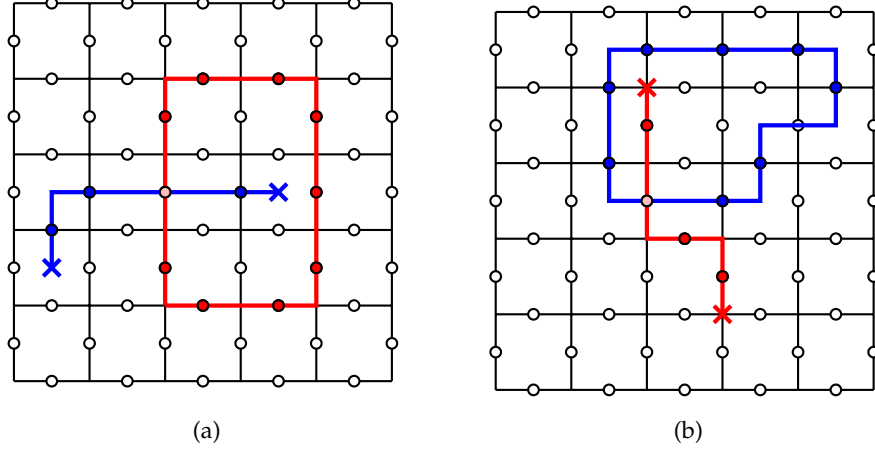
FIG. 5. Detection of defects using Wilson loops. (a) A magnetic defect is detected using a Wilson loop of star operators. (b) An electric defect is detected using a Wilson loop of plaquette operators.
